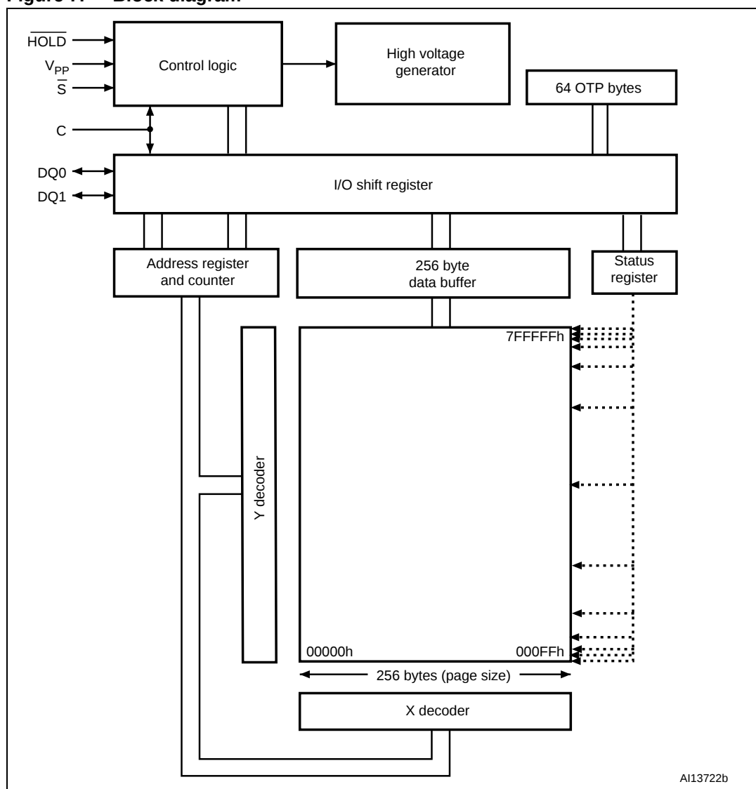
Figure 7. Block diagram
