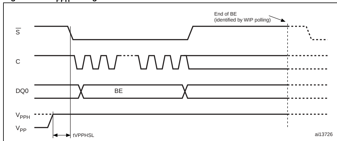
Figure 34. V_{PPH} timing
