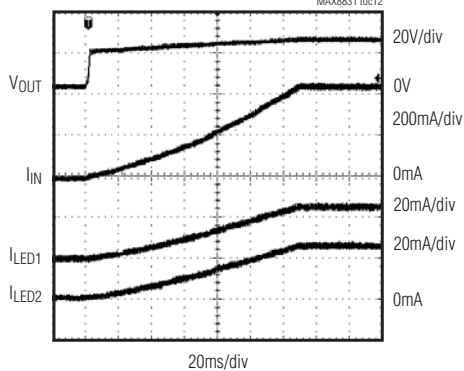
SOFT-START RESPONSE MAX8831 ttc12
