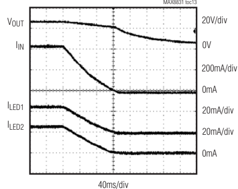
SHUTDOWN RESPONSE MAX8831 ttc13
