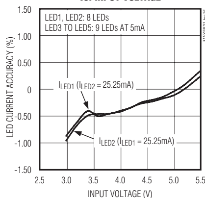
LED1, LED2 CURRENT ACCURACY vs. INPUT VOLTAGE MAX8831 ttc15
