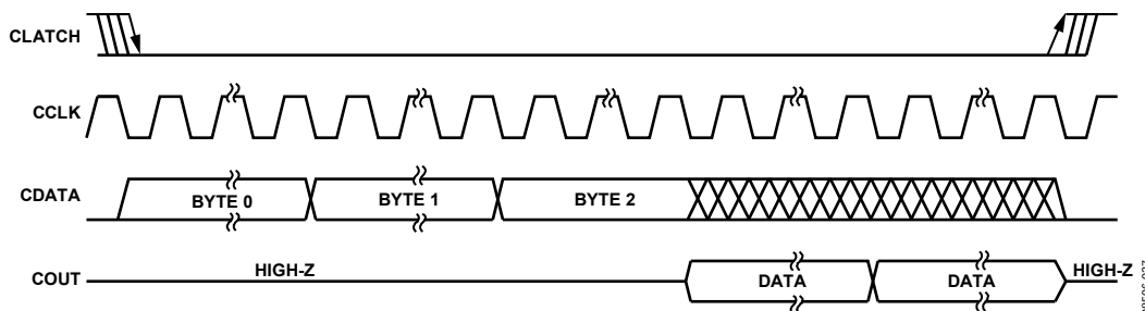
Figure 27. SPI Read from ADAU1401A Clcking (Single-Read Mode)
