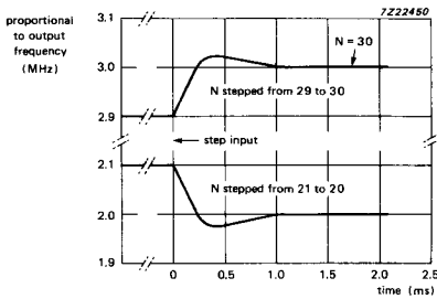
Fig. 34 Frequency compared to the time response.
