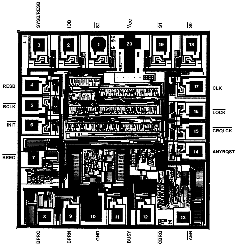
82C89
