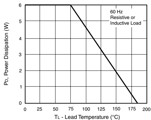
Figure 6. Power Derating Curve
