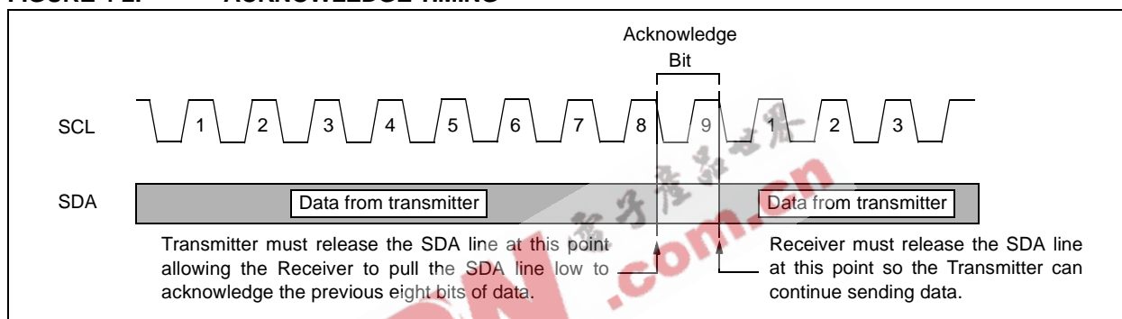
FIGURE 4-2: ACKNOWLEDGE TIMING
