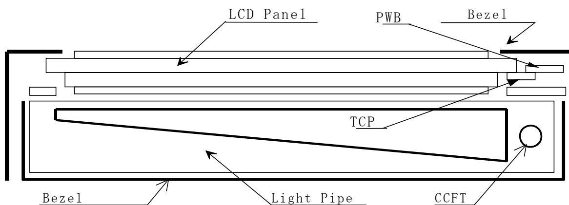
Fig.2 Module structure
