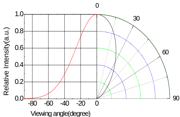
Radiation Characteristics
