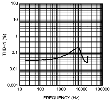
THD+N vs Frequency V_{DD} = 3.6V , P_{OUT} = 100mW , R_L = 4\Omega DAC Input, Internal Reference, Speaker Mode
