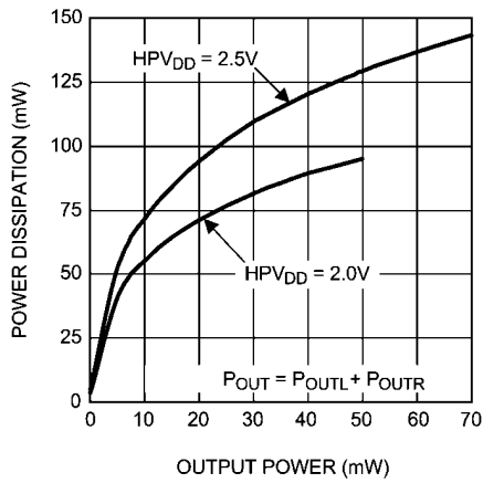
Power Dissipation vs Output Power R_L = 16\Omega , f = 1\text{kHz} , Headphone Mode
