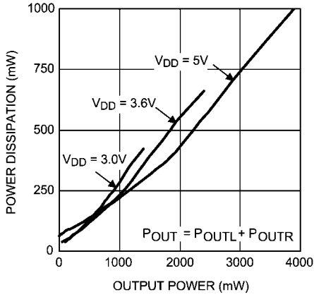
Power Dissipation vs Output Power R_L = 4\Omega , f = 1\text{kHz} , Speaker Mode
