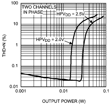
THD+N vs Output Power A_V = 20\text{dB} , R_L = 16\Omega , f = 1\text{kHz} DAC Input, Internal Reference, Headphone Mode
