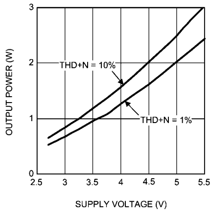
Output Power vs Supply Voltage R_L = 4\Omega , f = 1\text{kHz} , Speaker Mode
