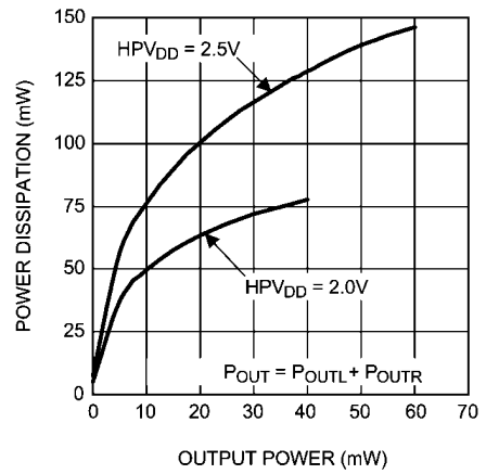
Power Dissipation vs Output Power R_L = 32\Omega , f = 1\text{kHz} , Headphone Mode
