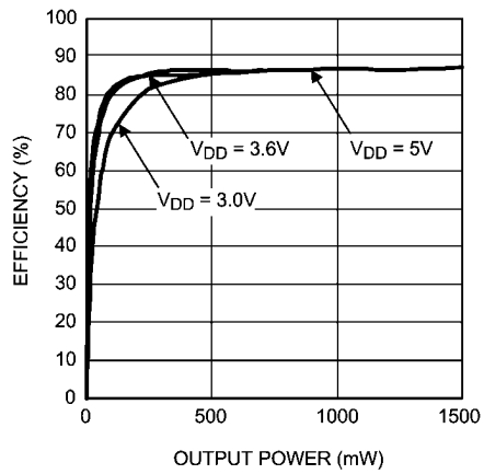
Efficiency vs Output Power R_L = 8\Omega , f = 1kHz , Speaker Mode
