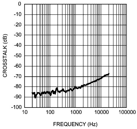
Crosstalk vs Frequency V_{DD} = 2.5V, V_{RIPPLE} = 1V_{P-P}, R_L = 8\Omega Analog Input, Speaker Mode
