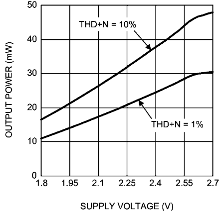
查询LM49450供应商 Output Power vs Supply Voltage R_L = 16\Omega, f = 1\text{kHz} , Headphone Mode
