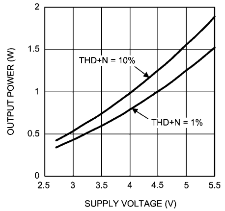
Output Power vs Supply Voltage R_L = 8\Omega , f = 1\text{kHz} , Speaker Mode
