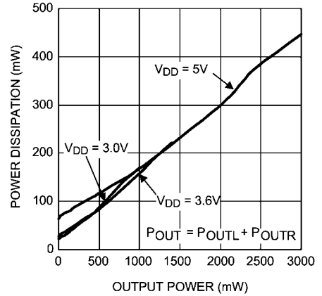
Power Dissipation vs Output Power R_L = 8\Omega , f = 1\text{kHz} , Speaker Mode
