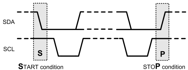
FIGURE 3. START and STOP Diagram
