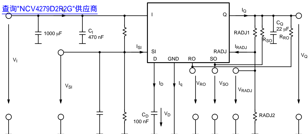
Figure 2. Measuring Circuit
