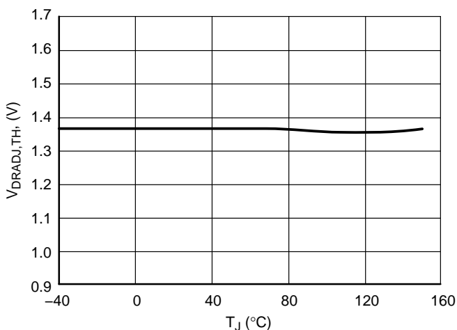
Figure 8. Reset Adjust Switching Threshold V_{DRADJ,TH} vs. Temperature T_J
