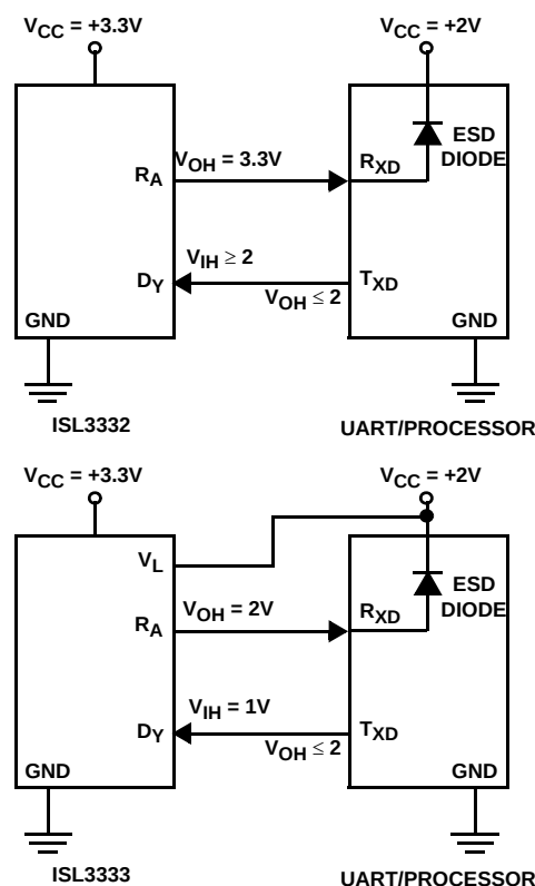
FIGURE 12. USING V_L PIN TO ADJUST LOGIC LEVELS
