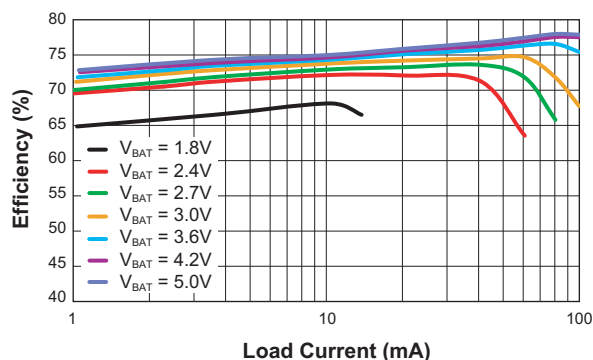
AUX3 Efficiency vs. Output Current ( V_{\text{AUX3}} = -7.5\text{V} ; L = 4.7\mu\text{H} ; C_{\text{OUT}} = 4.7\mu\text{F} )
