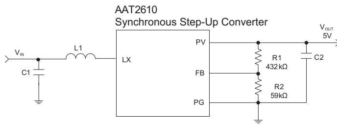
(a) Synchronous step-up converter
