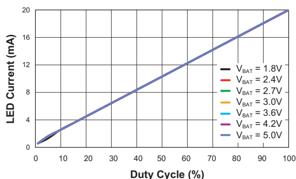
AUX1 PWM Duty Cycle vs. LED Current (4 WLEDs; L = 4.7\mu\text{H} ; C_{\text{OUT}} = 1\mu\text{F} ; 10kHz PWM Control)
