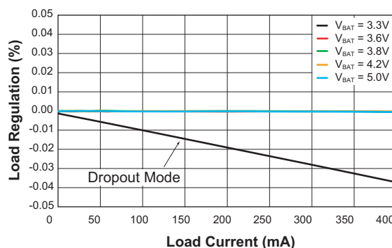
Main SD Load Regulation vs. Output Current ( V_{\text{PVM}} = V_{\text{BAT}} ; V_{\text{MSD}} = 3.3\text{V} ; L = 3.3\mu\text{H} ; C_{\text{OUT}} = 4.7\mu\text{F} )
