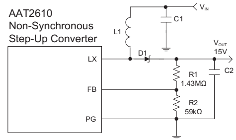
(b) Non-synchronous step-up converter
