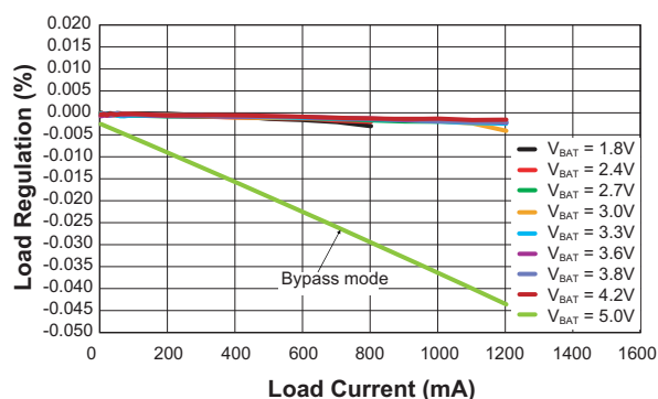
SU Load Regulation vs. Output Current ( V_{\text{SU}} = 5\text{V} ; L = 2.2\mu\text{H} ; C_{\text{OUT}} = 22\mu\text{F} )
