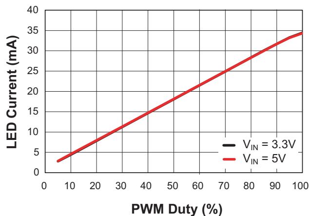
Figure 7: AUX1 Channel Application Example of Driving 4 WLEDs with Maximum 35mA Led Current.
