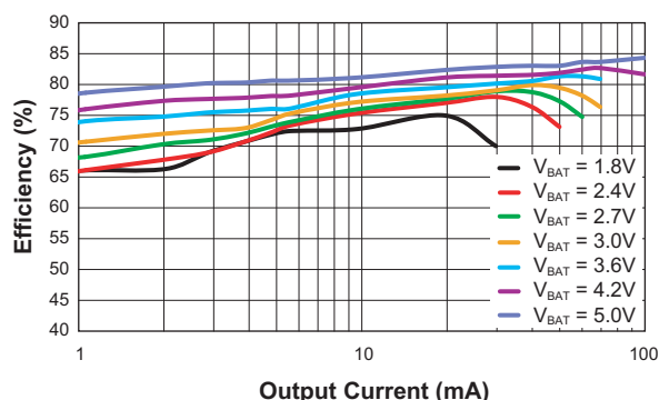
AUX2 Efficiency vs. Output Current ( V_{\text{AUX2}} = +15\text{V} ; L = 4.7\mu\text{H} ; C_{\text{OUT}} = 4.7\mu\text{F} )
