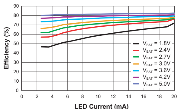
AUX1 Efficiency vs. PWM Duty Cycle (4 WLEDs; L = 4.7\mu\text{H} ; C_{\text{OUT}} = 1\mu\text{F} ; 10kHz PWM Control)
