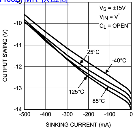
Negative Output Swing vs. Sinking Current 查询"LMH6321MR"供应商
