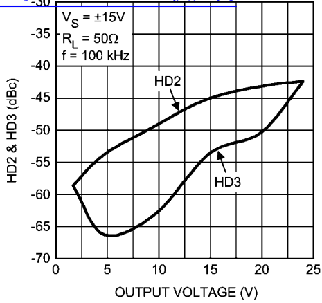
Harmonic Distortion with 50Ω Load 查询"LMH6321MR"供应商
