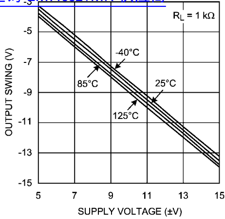
Negative Output Swing vs. Supply Voltage 查询"LMH6321MR"供应商
