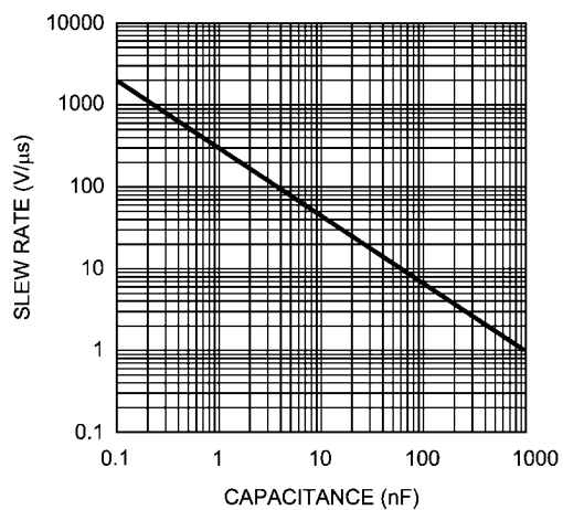
FIGURE 8. Slew Rate vs. Load Capacitance
