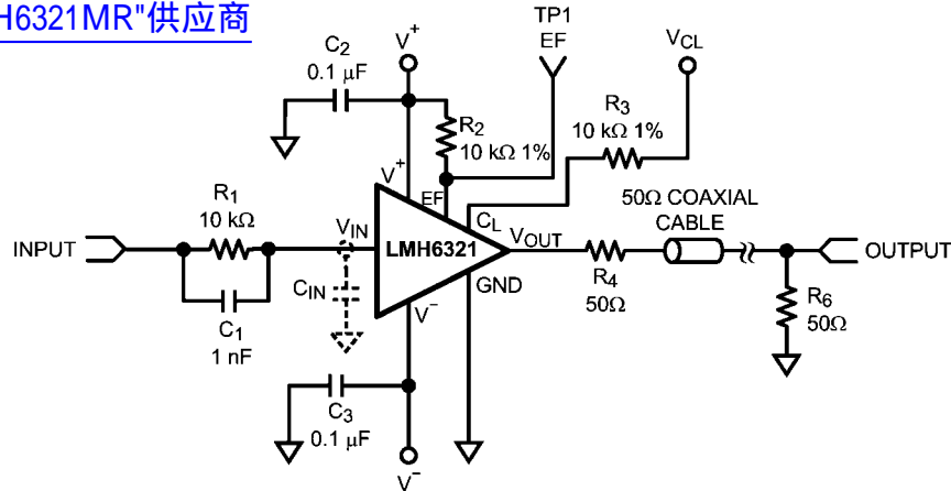
FIGURE 2. 50Ω Coaxial Cable Driver with Dual Supplies
