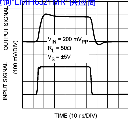
Small Signal Step Response 查询"LMH6321MR"供应商
