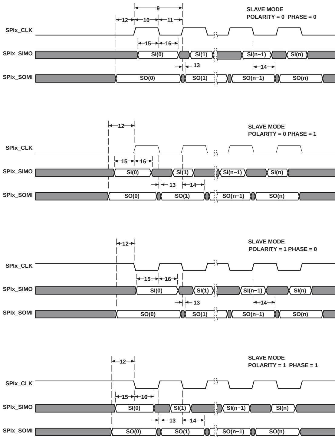
Figure 6-32. SPI Timings—Slave Mode
