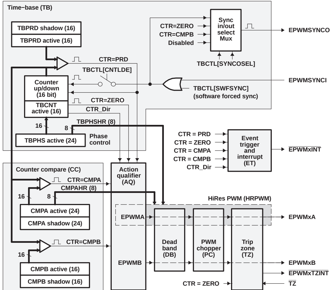
Figure 6-38. eHRPWM Sub-Modules Showing Critical Internal Signal Interconnections
