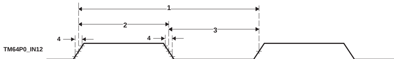
Figure 6-40. Timer Timing
