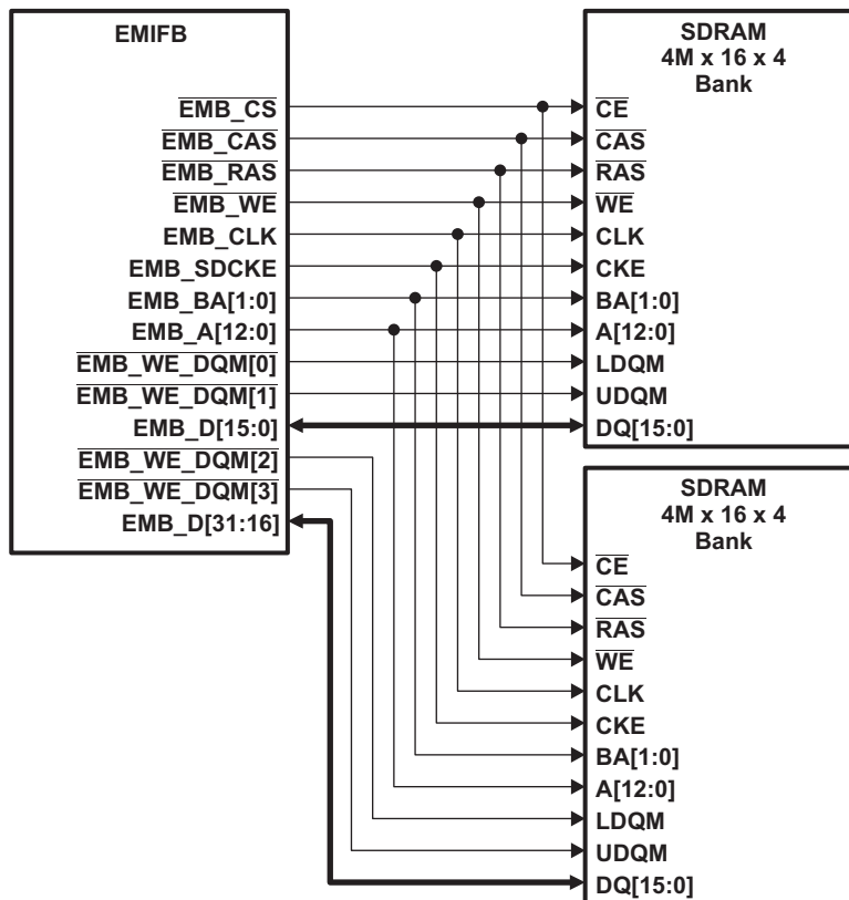
Figure 6-18. EMIFB to Dual 4M × 16 × 4 bank SDRAM Interface
