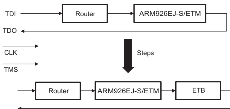
Figure 6-48. Adding ETB to the scan chain
