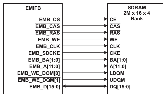
Figure 6-17. EMIFB to 2M × 16 × 4 bank SDRAM Interface
