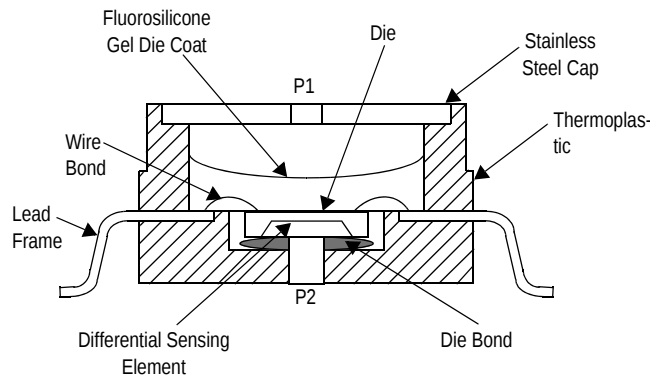
Figure 2. Cross Sectional Diagram SSOP (not to scale)
