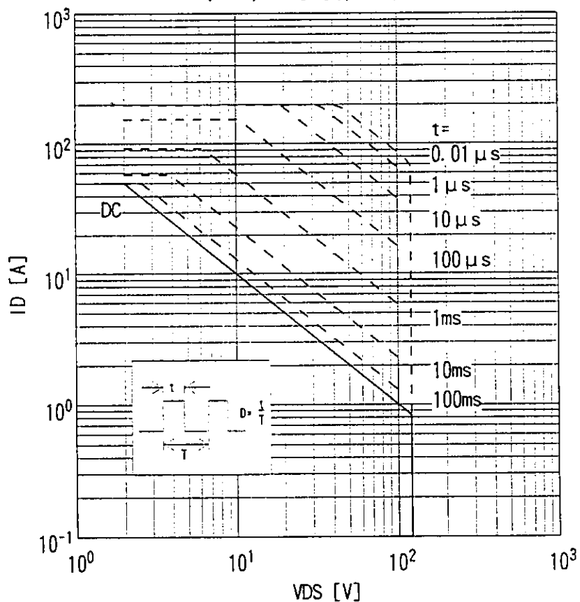
Safe operating area ID=f(V_{DS}):D=0.01, T_c=25^\circ\text{C}
