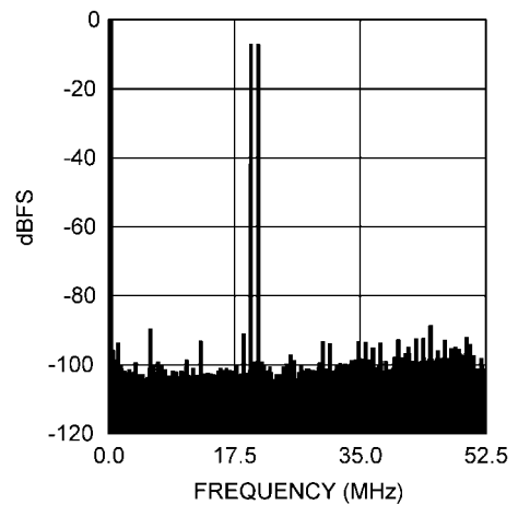
Intermodulation Distortion, f_{IN1} = 19.5 MHz, f_{IN2} = 20.5 MHz
