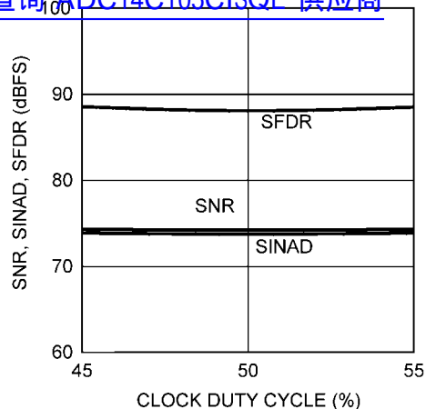
SNR, SINAD, SFDR vs. Clock Duty Cycle 查询"ADC14C105CISQF"供应商
