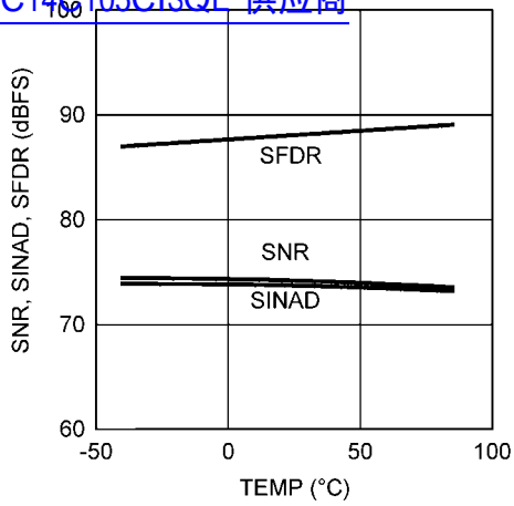
SNR, SINAD, SFDR vs. Temperature 查询"ADC14C105CISQF"供应商
