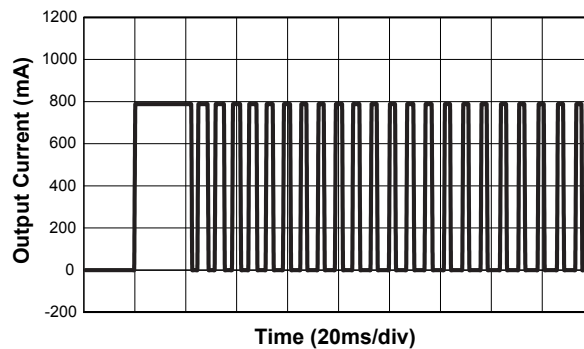
Over-Current Protection
