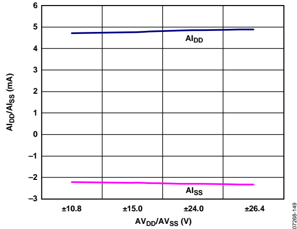
Figure 49. A_{I_{DD}}/A_{I_{SS}} vs. AV_{DD}/AV_{SS} , V_{OUT} = 0\text{ V}
