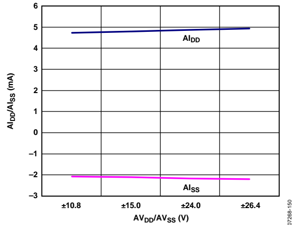
Figure 50. A_{I_{DD}}/A_{I_{SS}} vs. AV_{DD}/AV_{SS} , I_{OUT} = 0\text{ mA}
