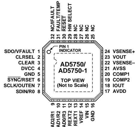
Figure 4. Pin Configuration
