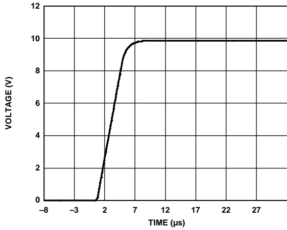
Figure 17. Full-Scale Positive Step
