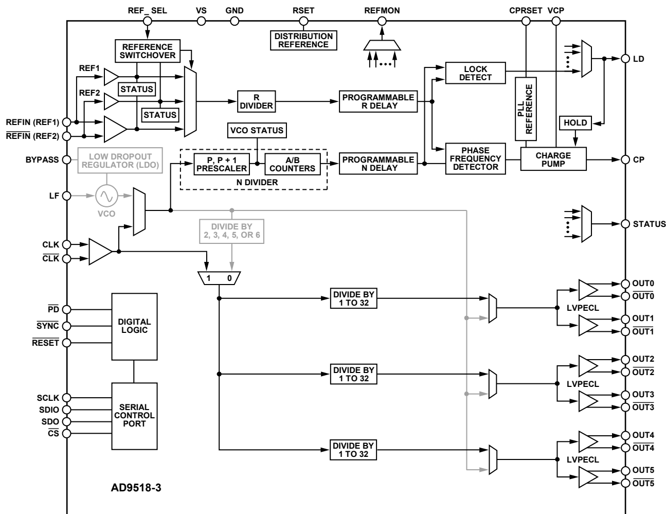
Figure 29. Clock Distribution or External VCO < 1600 MHz
