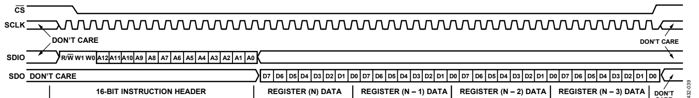
Figure 46. Serial Control Port Read—MSB First, 16-Bit Instruction, Four Bytes Data
