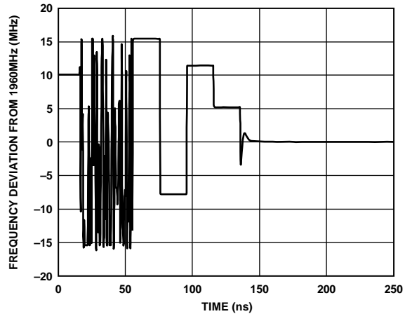
Figure 22. Frequency Deviation from LO Frequency at LO = 1.97 GHz to 1.96 GHz vs. Lock Time
