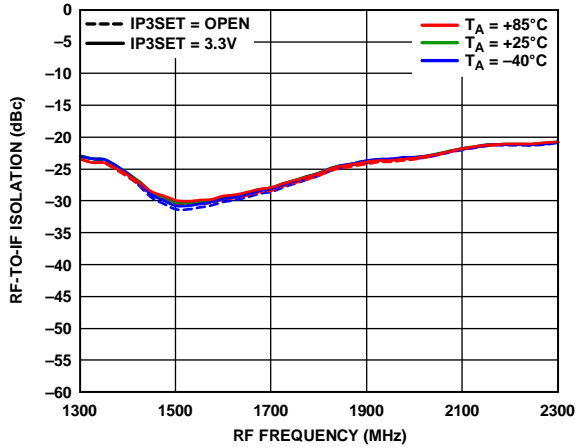
Figure 20. RF-to-IF Leakage vs. RF Frequency, High-Side LO, IF = 140 MHz, LO Output Turned Off
