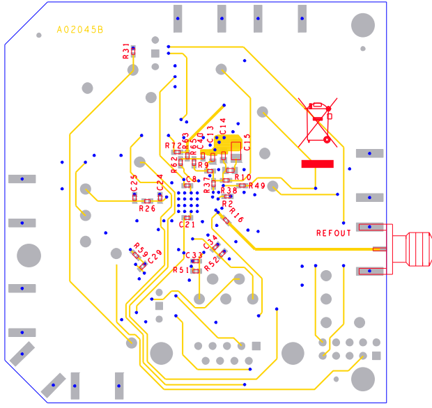
Figure 51. Evaluation Board Layout (Bottom)
