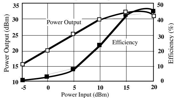
Power Output & Power Added Efficiency vs Power Input 850 MHz, V_{DS} = 8\text{ V} , I_{DS} = 400\text{ mA}
