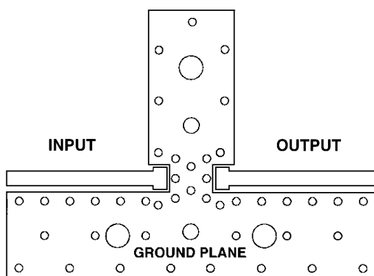
BOARD LAYOUT
