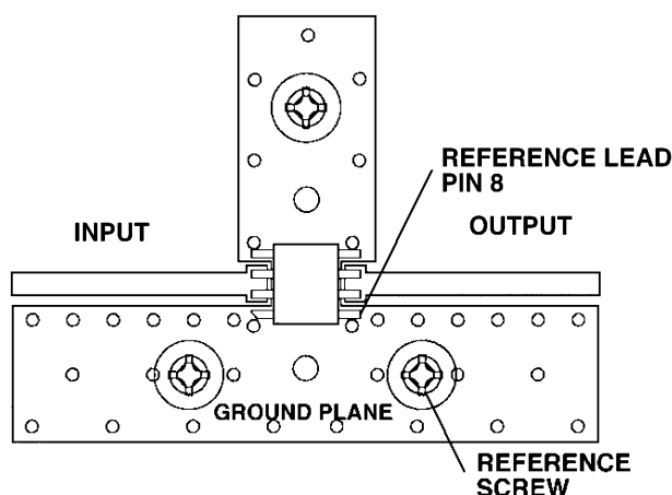
THERMAL MOUNTING DIAGRAM
