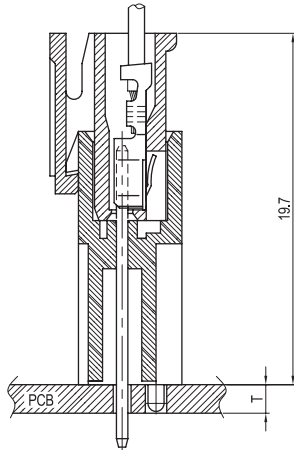
PCB ASSY
