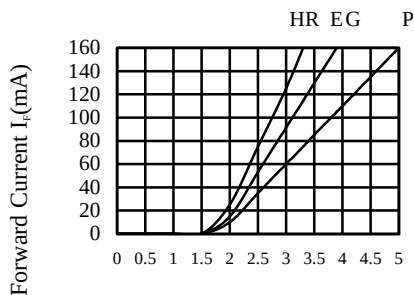
FIG.4 FORWARD CURRENT VS. FORWARD VOLTAGE
