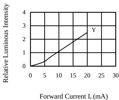
FIG.2-1 RELATIVE LUMINOUS INTENSITY VS. FORWARD CURRENT
