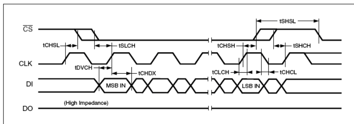
Figure 24. Input Timing
