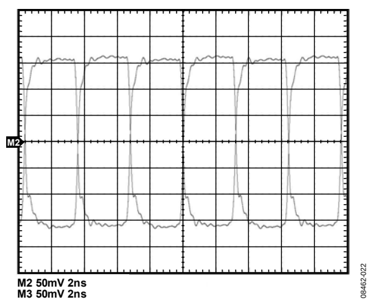
Figure 13. 156.25 MHz LVDS Output
