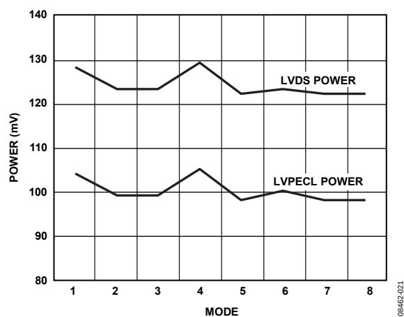
Figure 12. Typical Power Dissipation vs. Mode
