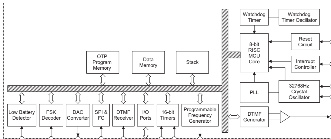
Block Diagram
