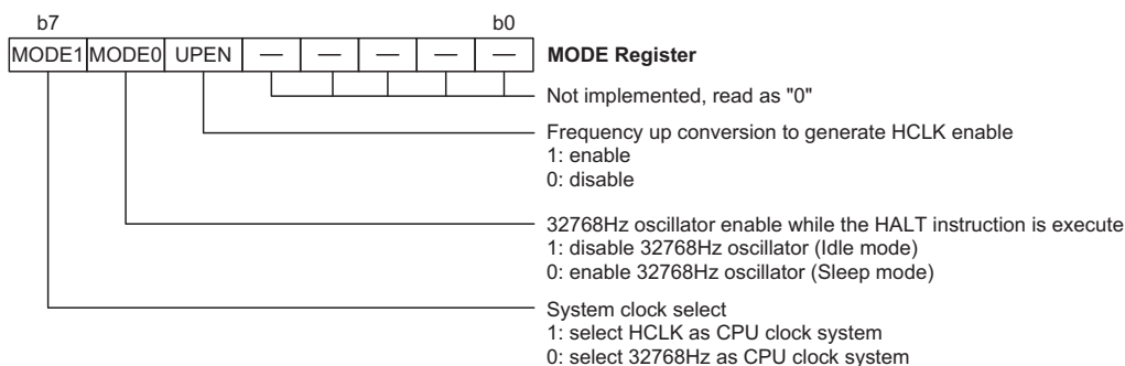
MODE Register
