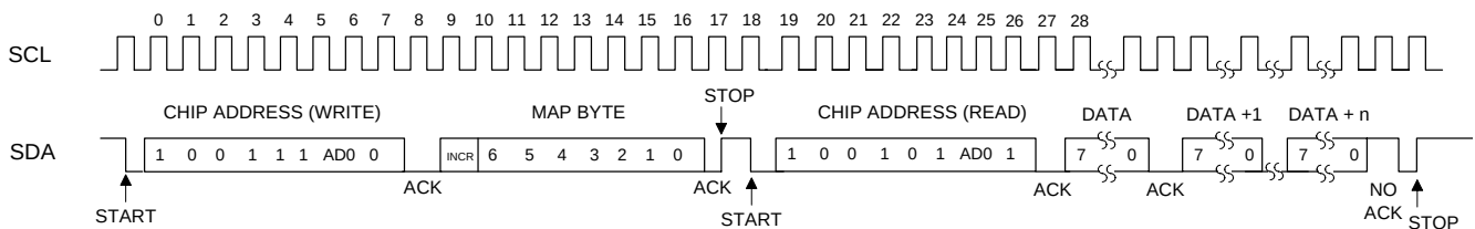
Figure 19. Control Port Timing, I²C Aborted Write + Read
