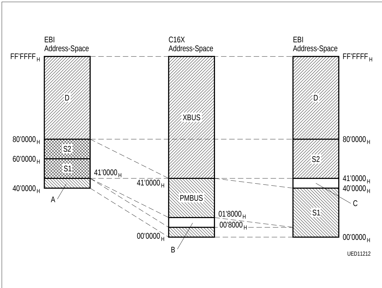
Figure 4-8 Memory Mapping
