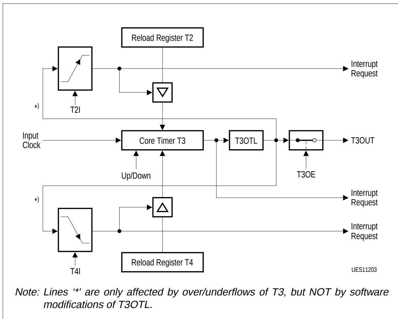
Figure 7-12 GPT1 Timer Reload Configuration for PWM Generation
