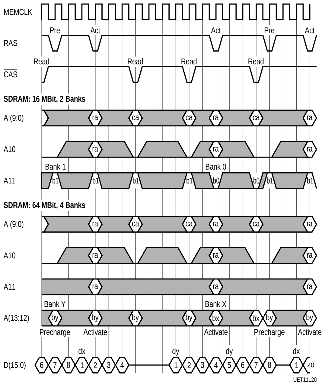
Figure 4-7 Interlocked Access Cycles to two SDRAM Banks
