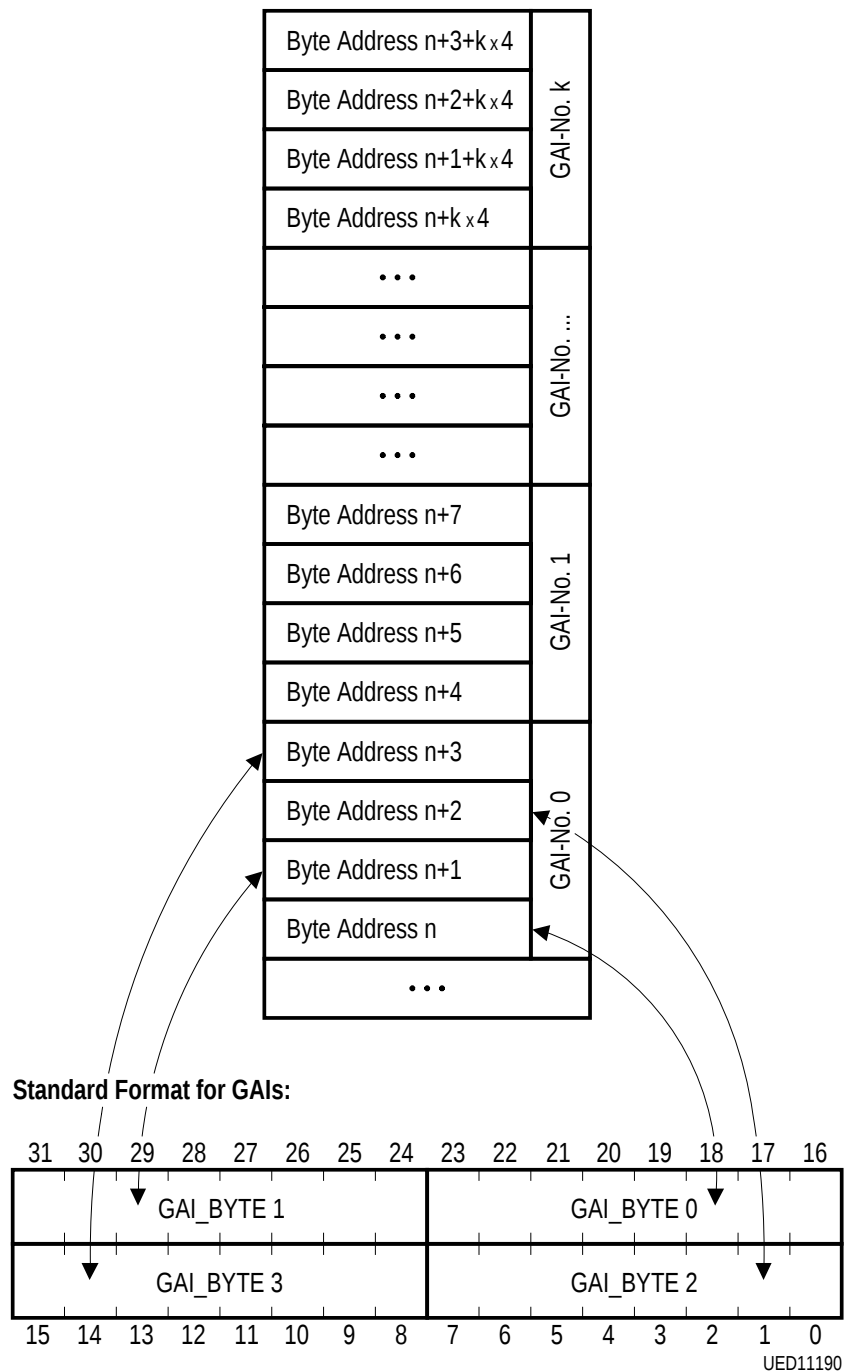
Figure 10-21 Organization of GAIs in the External SDRAM
