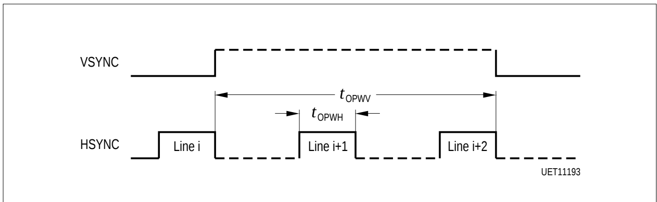
Figure 14-1 H/V - Sync-Timing (Sync-master mode)
