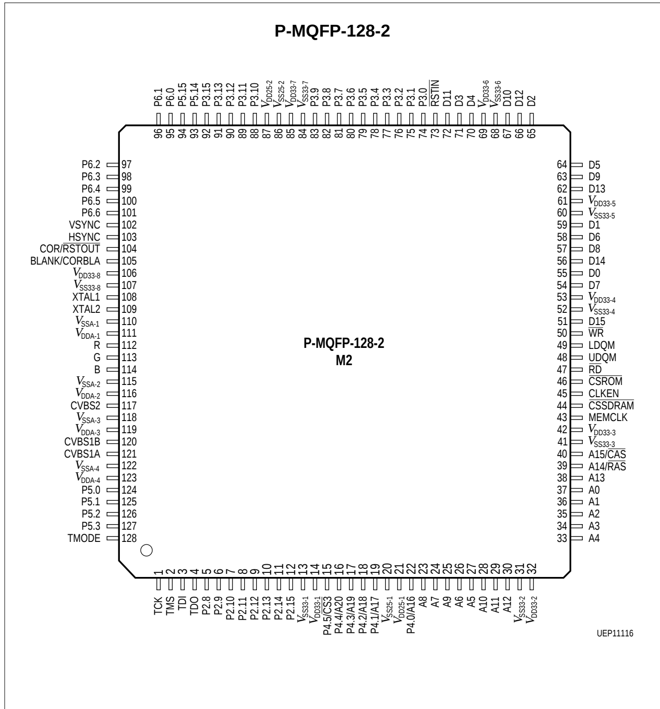
Figure 2-1 Pin Configuration
