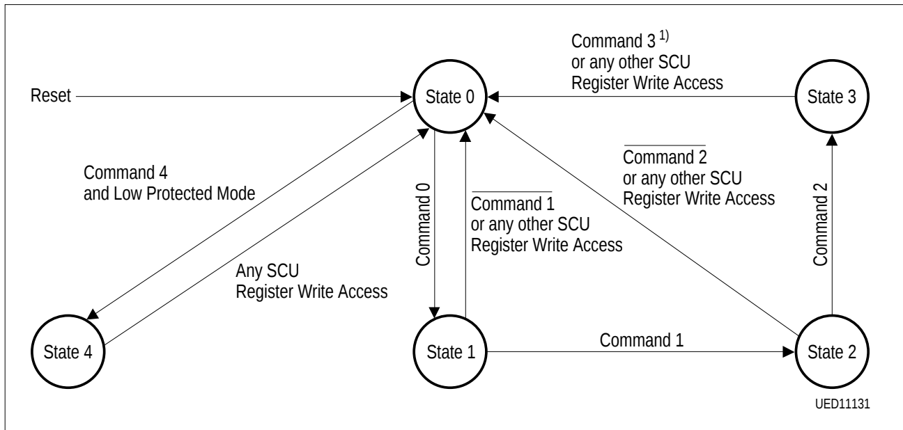
Figure 6-1 State Machine for Security Level Switching
