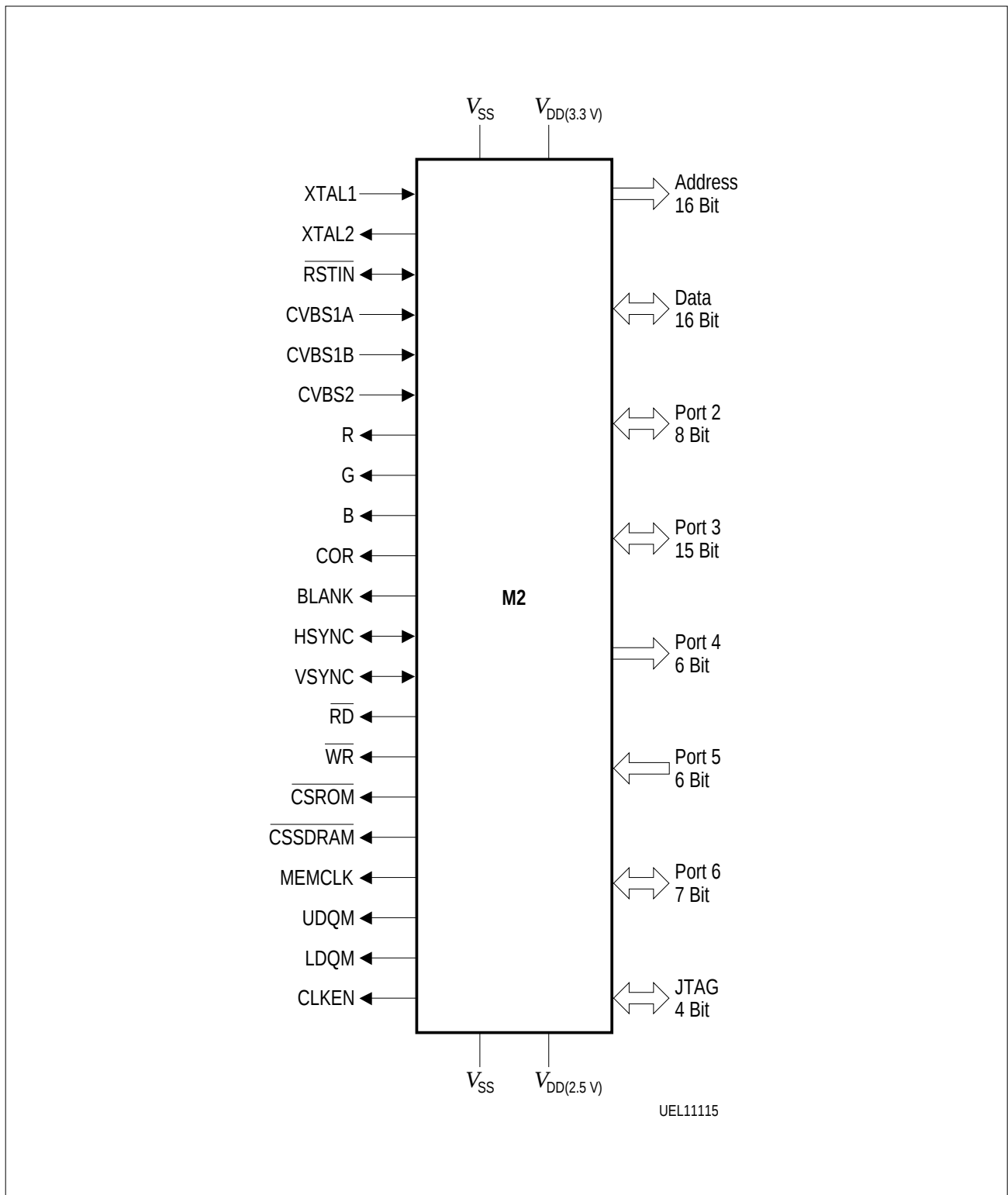
Figure 1-2 Logic Symbol
