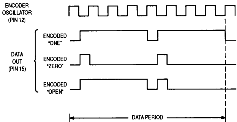
Figure 11. Encoder Data Waveforms
