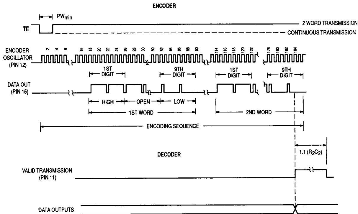
Figure 10. Timing Diagram
