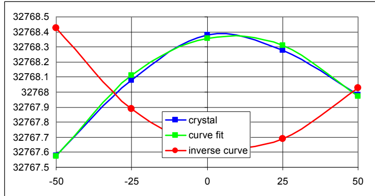
Figure 31: Crystal Compensation
