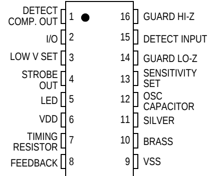
Figure 1. Pin Connections
