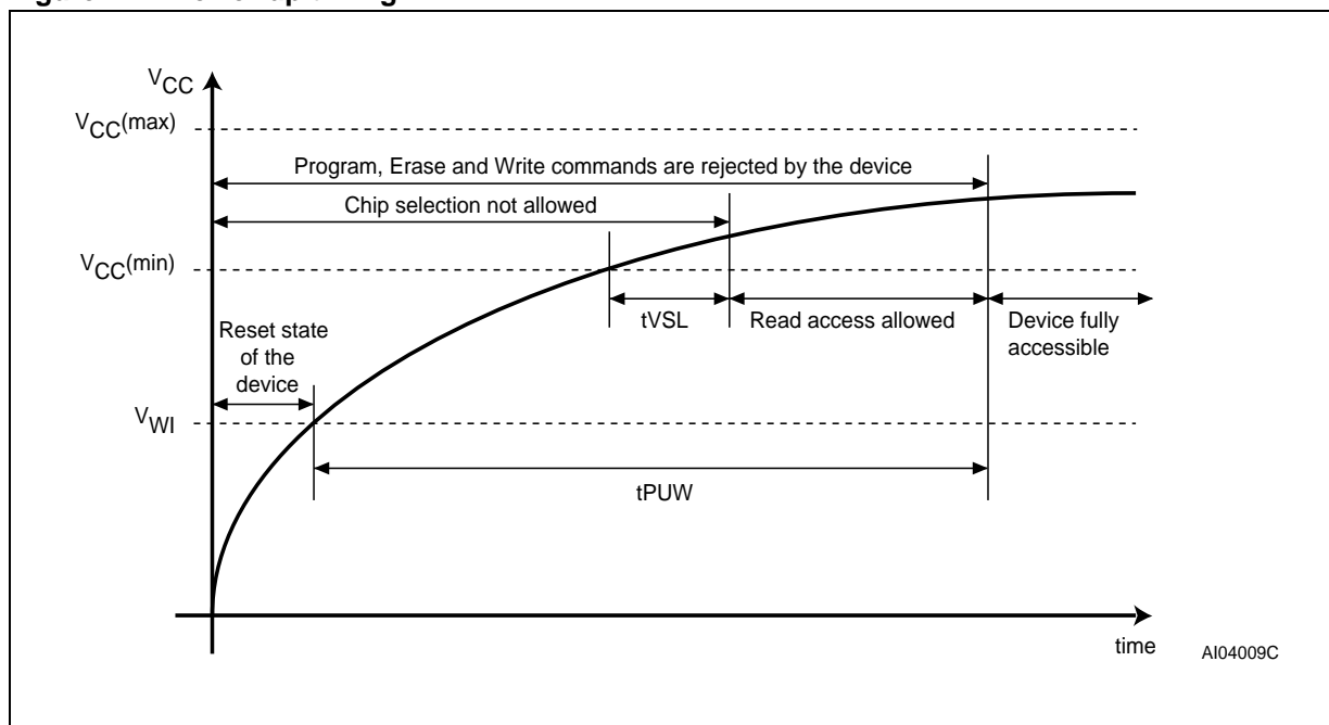
Figure 24. Power-up timing
