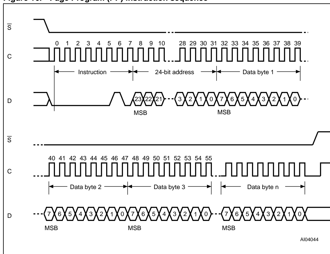
Figure 16. Page Program (PP) instruction sequence
