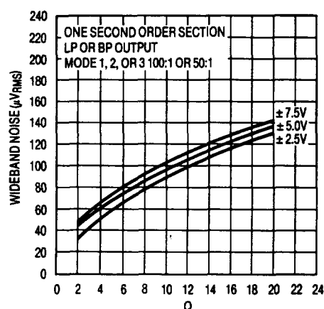
Graph 6. Wideband Noise vs Q
