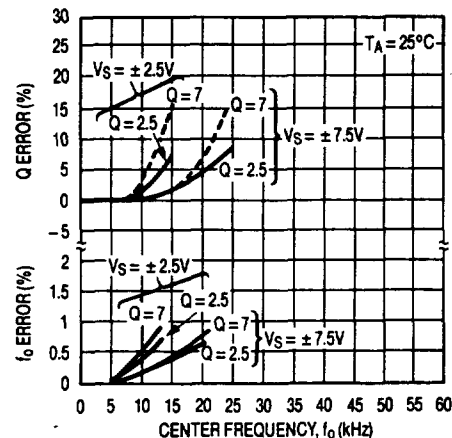
Graph 3. Mode 3, ( f_{CLK}/f_o ) = 50:1
