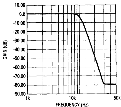
Graph 9. LTC1164 8th Order Butterworth, f_{CLK} = 500kHz , f_{-3dB} = 10kHz
