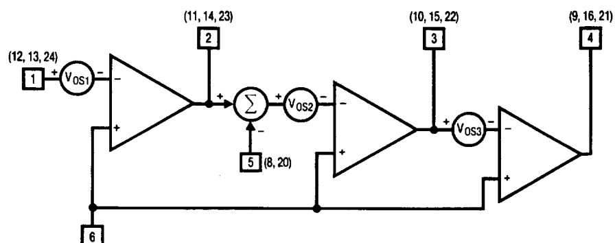
Figure 1. Equivalent Input Offsets of \frac{1}{4} LTC1164 Filter Building Block
