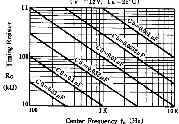
VCO Frequency
