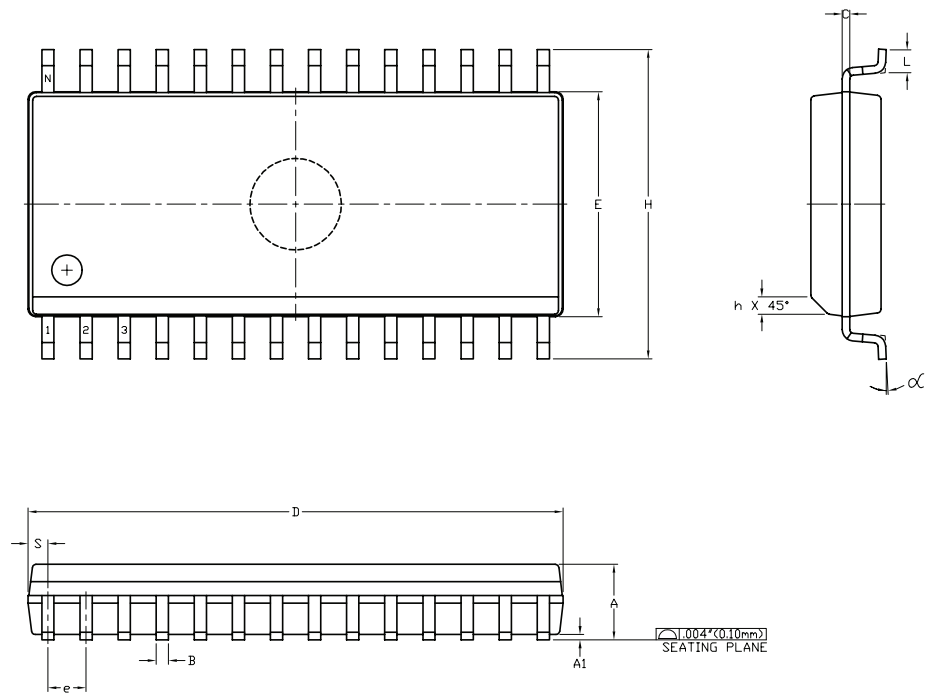
Figure 18-1. 28-Pin SOIC
