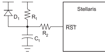
Figure 6-1. External Circuitry to Extend Reset
