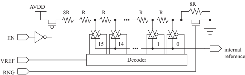
Figure 13-3. Comparator Internal Reference Structure
