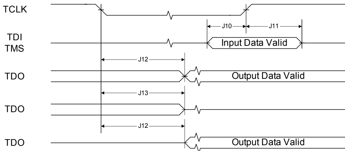
Figure 17-6. JTAG Test Access Port (TAP) Timing
