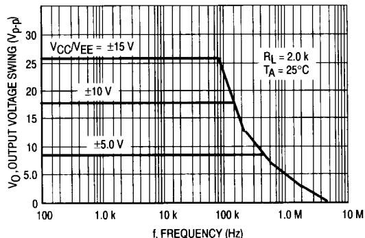
Figure 2. Output Voltage Swing versus Frequency
