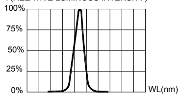
FIG.4 RELATIVE LUMINOUS INTENSITY VS. WAVELENGTH.
