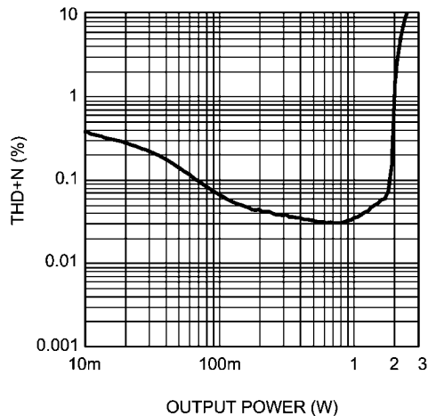
THD+N vs Output Power V_{DD} = 5.0V , R_L = 4\Omega , A_V = 6dB
