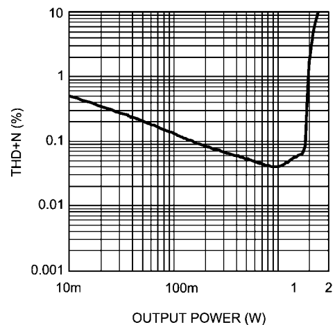
THD+N vs Output Power V_{DD} = 3.6V , R_L = 4\Omega , A_V = 24dB
