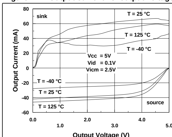
Figure 11. Output current vs. output voltage
