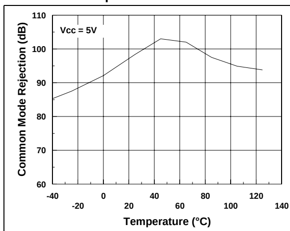
Figure 5. Common mode rejection vs. temperature
