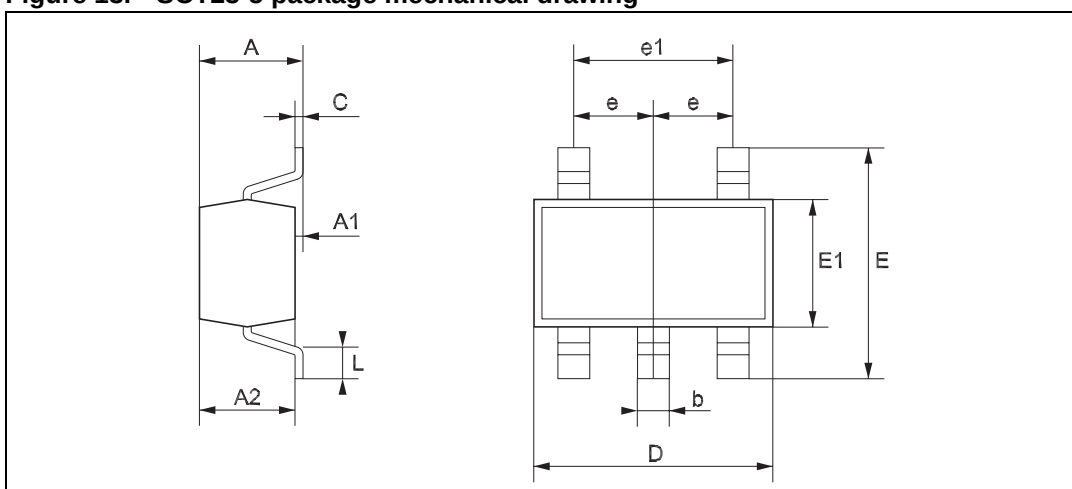
Figure 13. SOT23-5 package mechanical drawing
