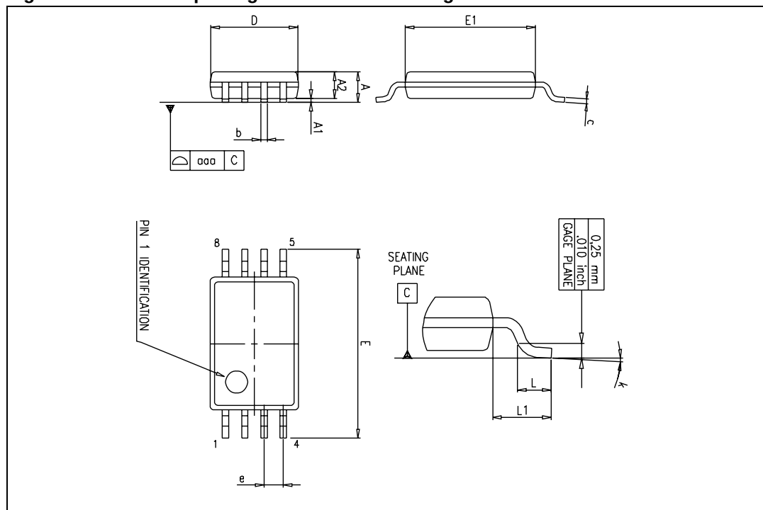
Figure 15. TSSOP8 package mechanical drawing
