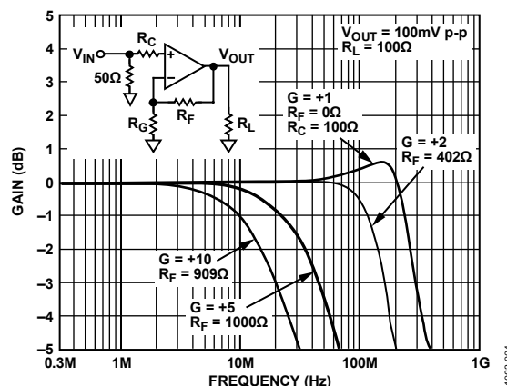
Figure 4. Frequency Response
