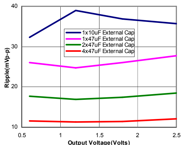
Figure 37. Output ripple voltage for various output voltages with external 1x10 \mu F, 1x47 \mu F, 2x47 \mu F or 4x47 \mu F ceramic capacitors at the output (20A load). Input voltage is 3.3V.
