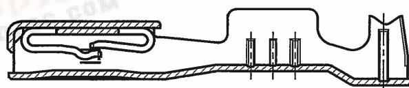
SECT. B-B (SCALE 5:1)
