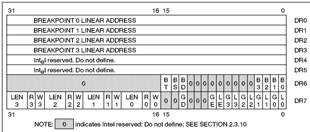
Figure 2-13. Debug Registers
