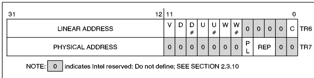
Figure 2-12. Test Registers
