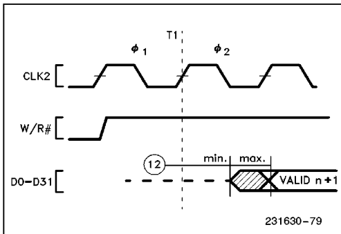
Figure 9-5a. Write Data Valid Delay Timing (25 MHz, 33 MHz)
