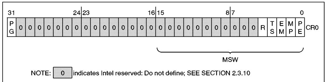
Figure 2-5. Control Register 0
