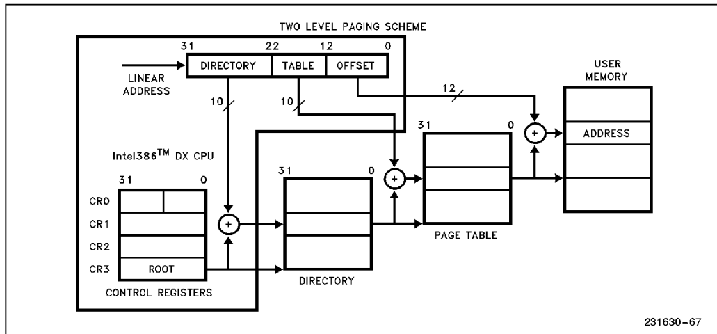
Figure 4-19. Paging Mechanism
