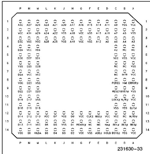
Figure 1-1. Intel386™ DX PGA Pinout—View from Top Side
