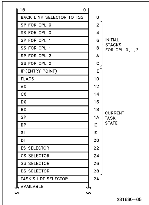
Figure 4-16. 80286 TSS
