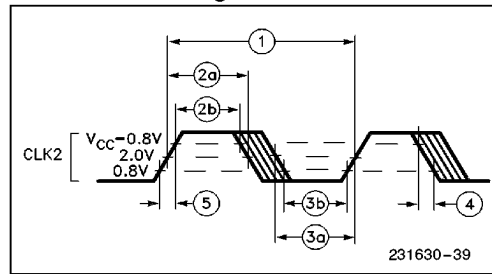
Figure 9-3. CLK2 Timing
