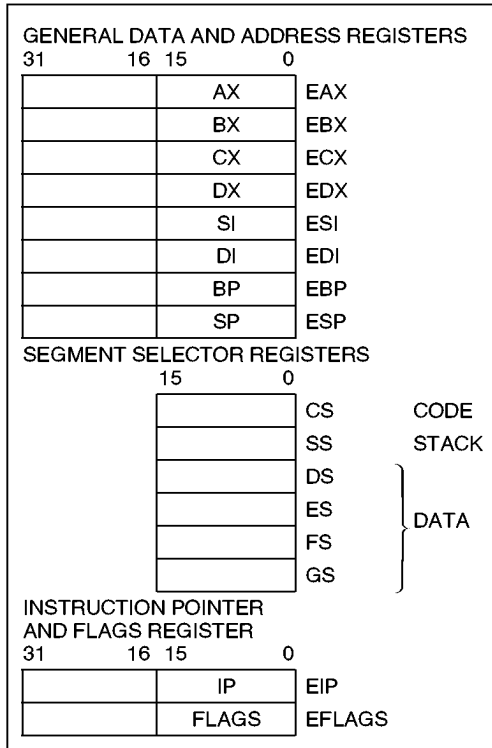
Figure 2-1. Intel386™ DX Base Architecture Registers
