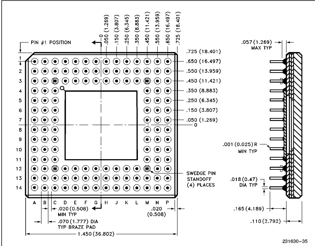
Figure 8.1. 132-Pin Ceramic PGA Package Dimensions
