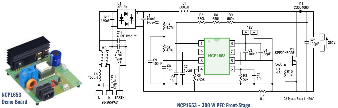
NCP1653 - 300 W PFC Front-Stage
