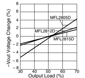
+Pout 80 to 20%, -Pout 20 to 80% Cross Regulation
