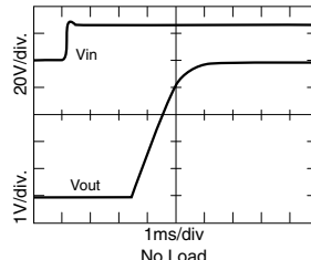
MFL2805S Turn On Response
