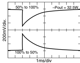
MFL2815D Step Load Response
