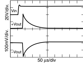
MFL2815D Step Line Response
