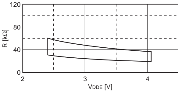
Pull-up resistor example characteristics Ta = +25 °C
