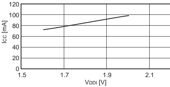
I CC -V DD1 example characteristics Ta = +25 °C, f CP = 68 MHz f CP = 34 MHz, f CP T = 34 MHz
