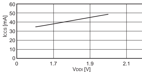
I CCS -V DDI example characteristics Ta = + 25 °C
