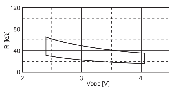
Pull-down resistor example characteristics T_a = +25\text{ }^\circ\text{C}
