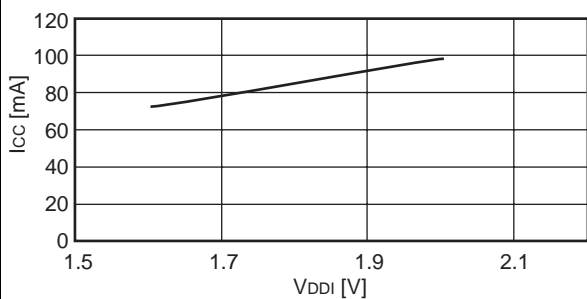
I CC -V DDI example characteristics Ta = + 25 °C, f CP = 68 MHz f CP = 34 MHz, f CPT = 34 MHz
