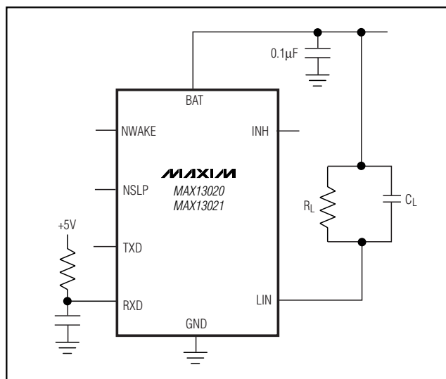
Figure 5. Test Circuit for AC Characteristics
