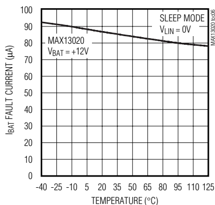
IBAT FAULT CURRENT vs. TEMPERATURE
