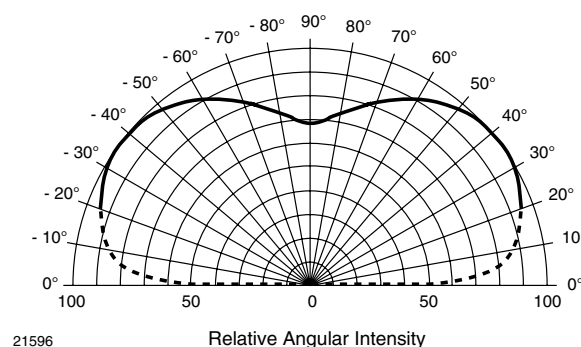
Fig. 2 - Radiant Characteristics I_{\text{rel}} = f(\varphi)
